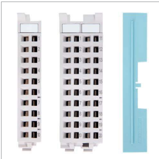
10-terminal front connector, 20-terminal front connector, final bus cover
