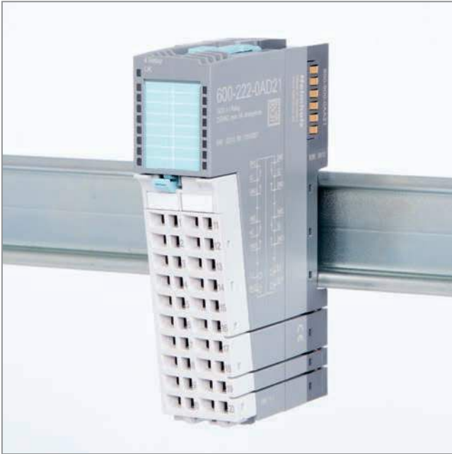
DO 4 x relays, 5 A, 230 VAC, changeover
